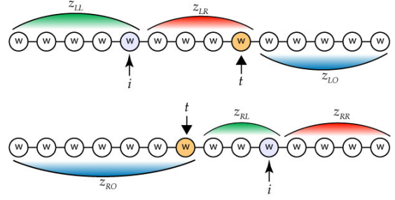
Figure 1: Sentence decomposition.
