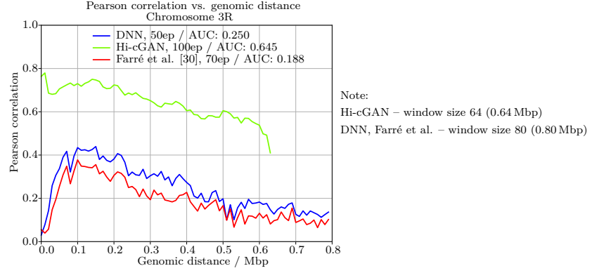
Figure 59: Comparison Pearson correlations per distance DNN / Hi-cGAN / Farré et al. [30]
