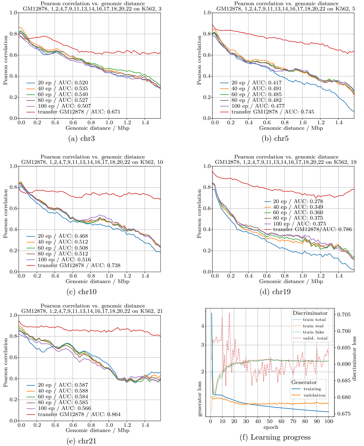
Figure 42: Results / metrics, cGAN, DNN embedding, no pre-training, w = 64 , test chromosomes
