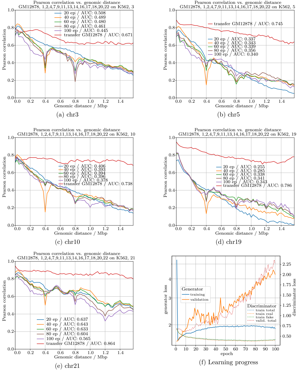
Figure 52: Results / metrics, cGAN, mixed embedding, no pre-training, w = 64 , test chromosomes
