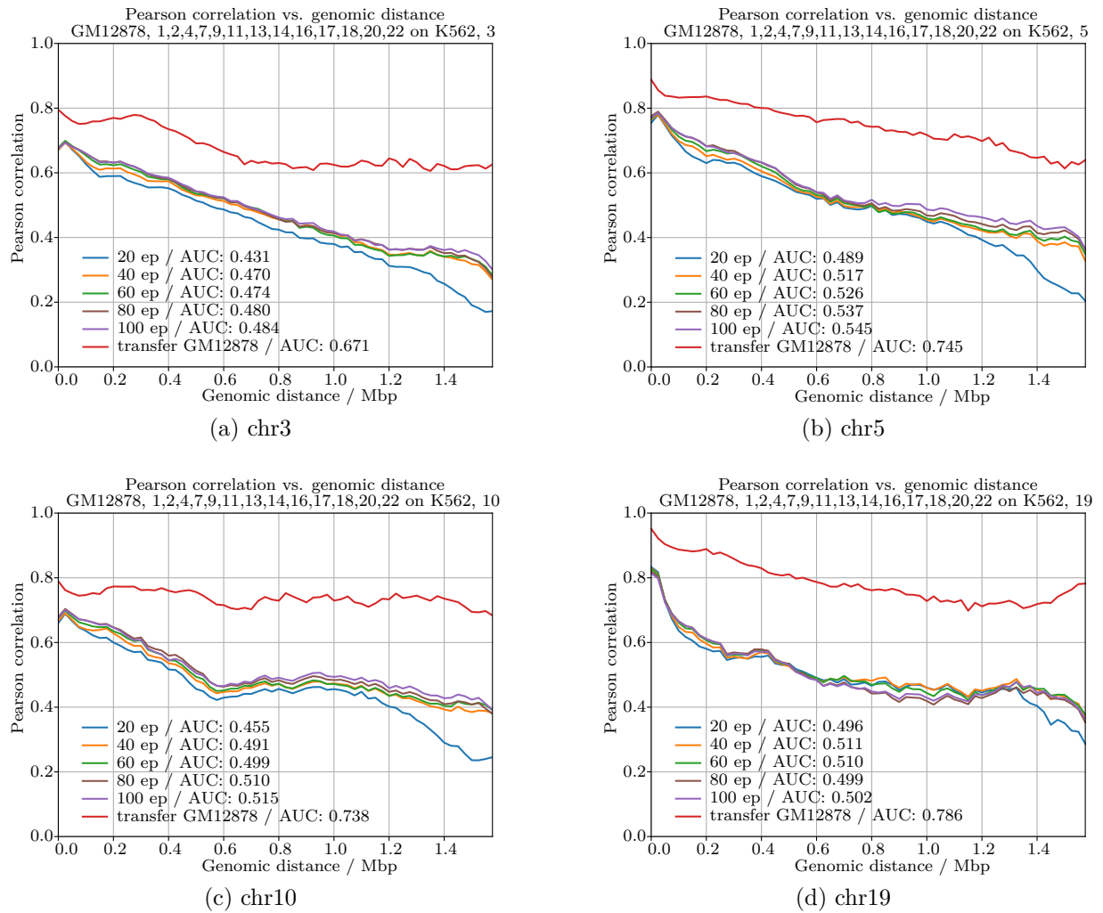
Figure 66: Results / metrics, cGAN, w = 64 , trained on GM12878 chr14 only; prediction on K562, typical test chromosomes
