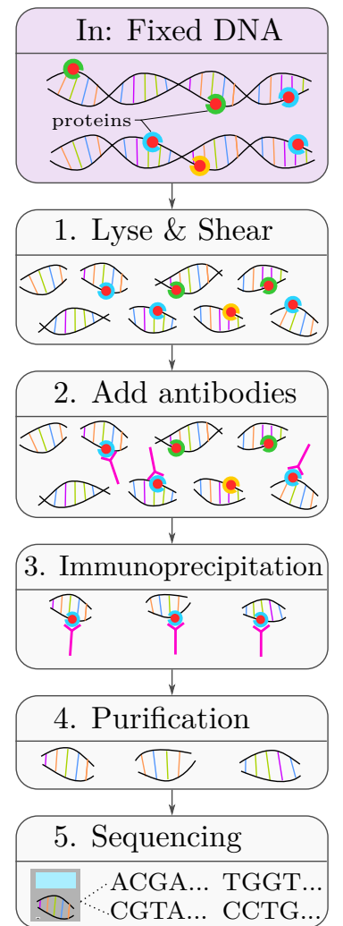
Figure 3: ChIP-seq lab process
