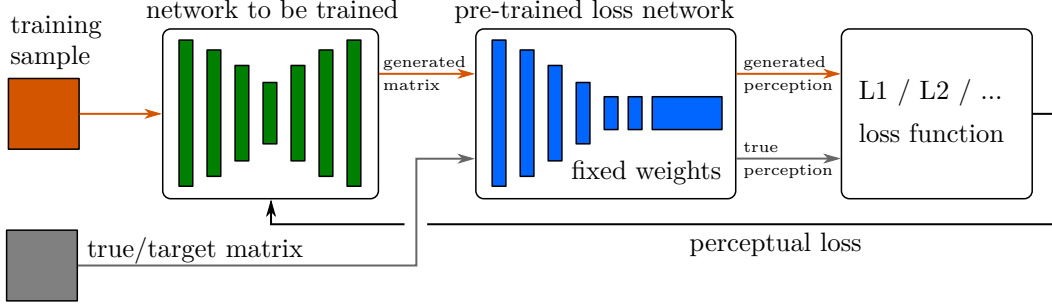
Figure 5: Perceptual loss
