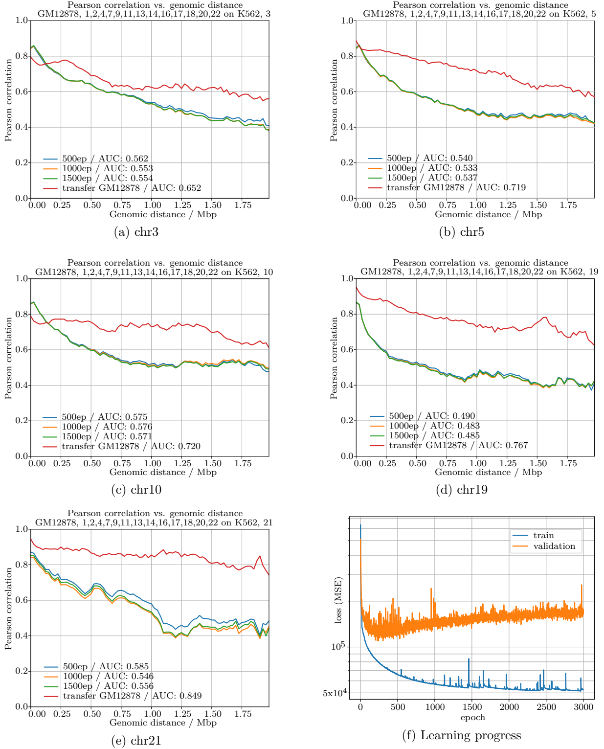
Figure 20: Results / metrics, basic DNN, 25 kbp, test chromosomes
