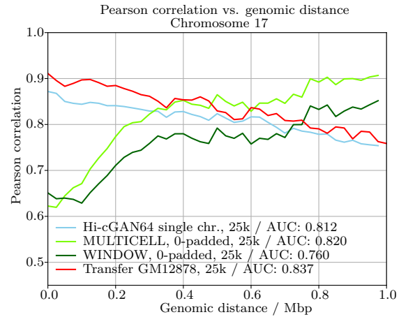
(f) Hi-cGAN single chrom: chr17 detail 0...1 Mbp
