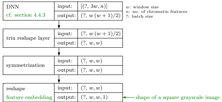
Figure 17: Embedding network, DNN
