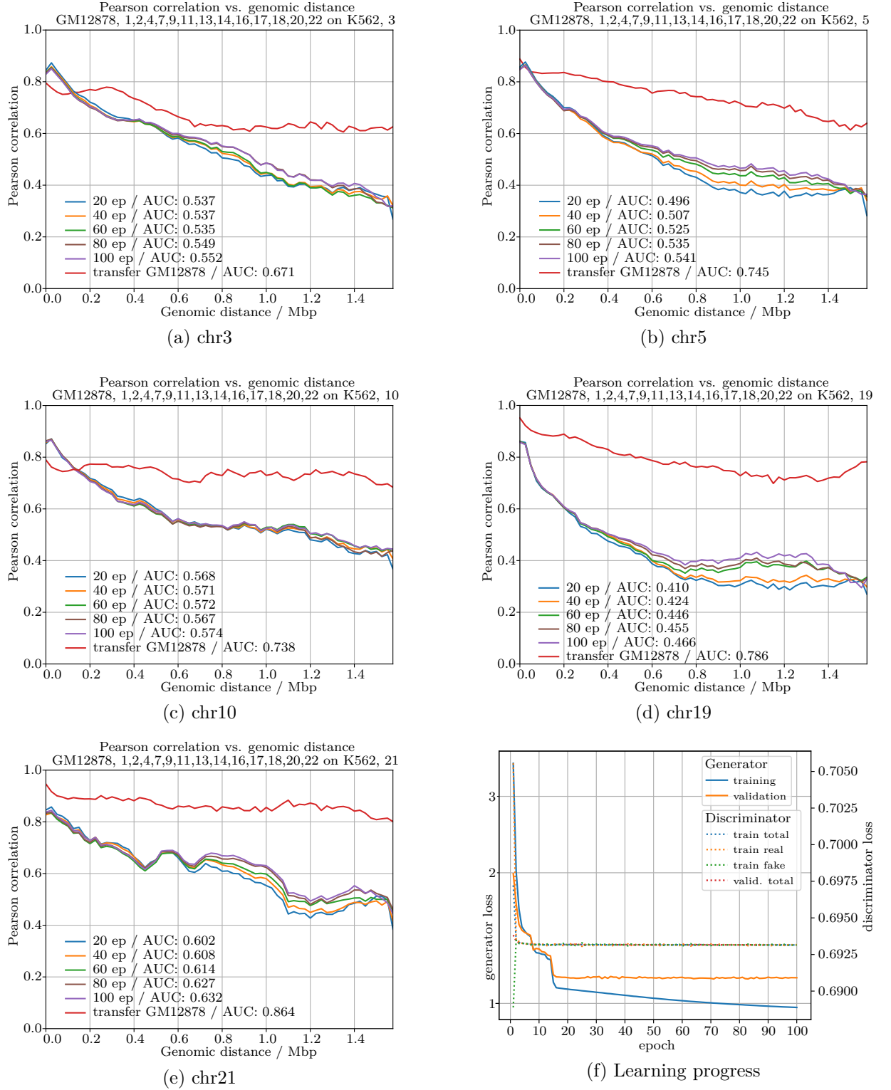
Figure 44: Results / metrics, cGAN, DNN embedding, pre-trained, w = 64 , test chromosomes
