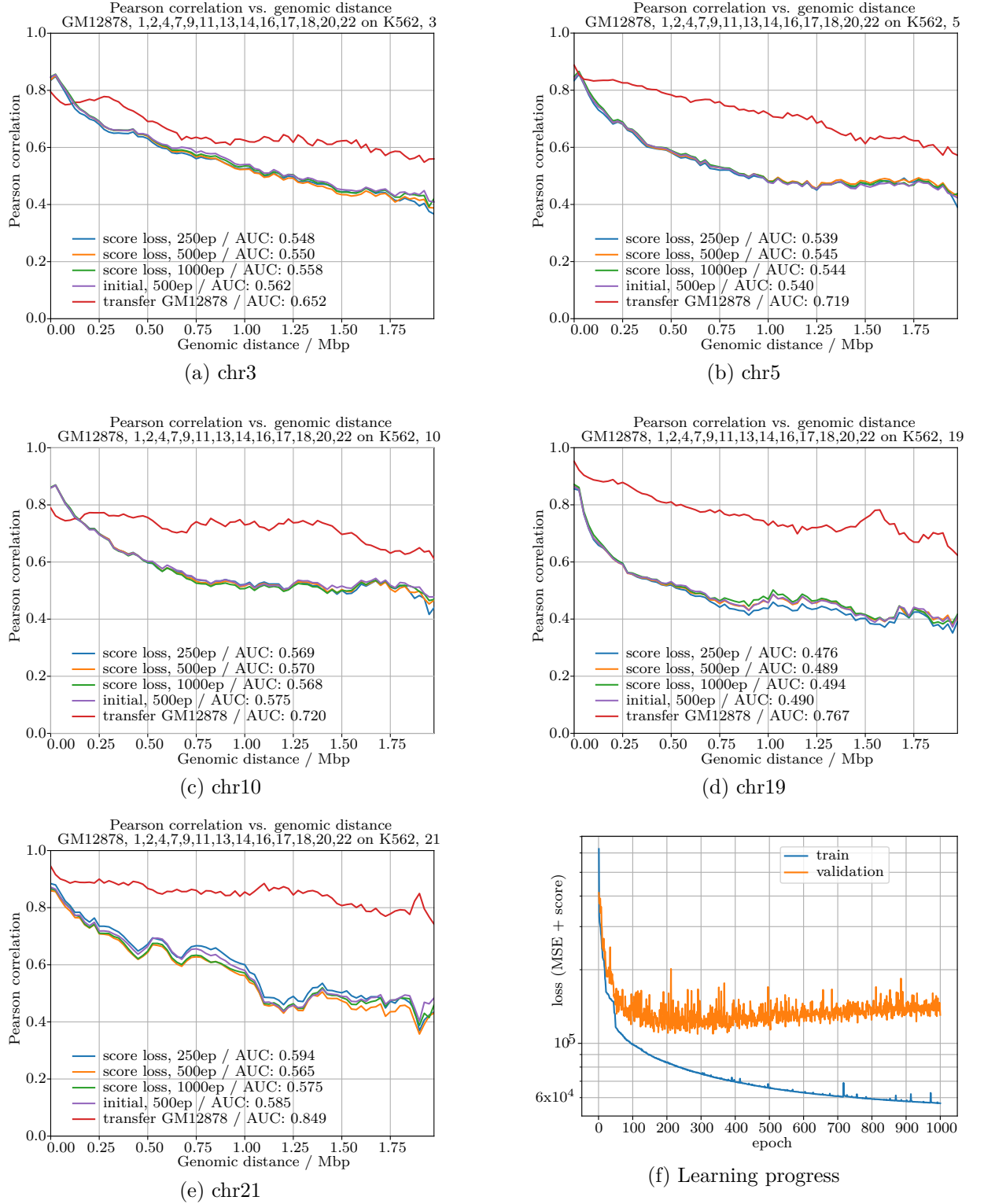
Figure 35: Results / metrics, DNN with score-based loss function, test chromosomes (\lambda_{MSE} = 1.0, \lambda_{score} = 100, ds = 12)
