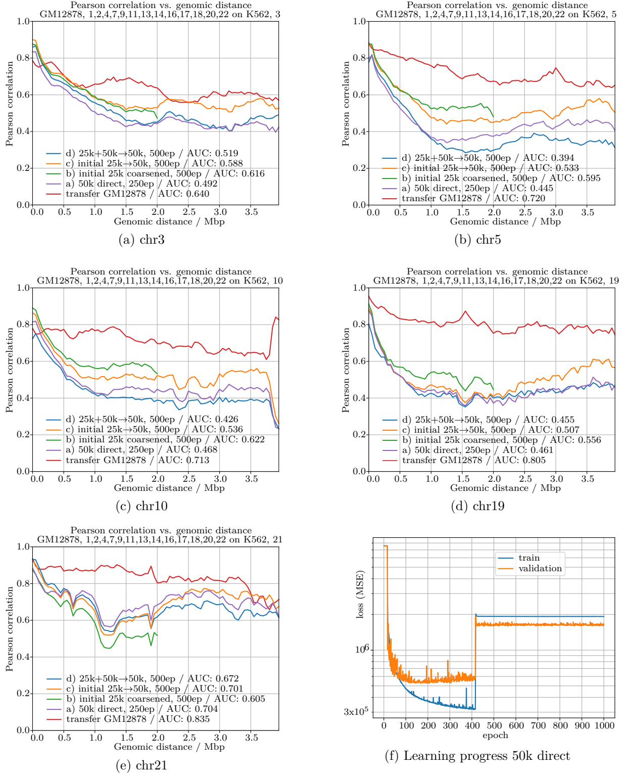
Figure 37: Results / metrics, various DNNs at 50kbp
