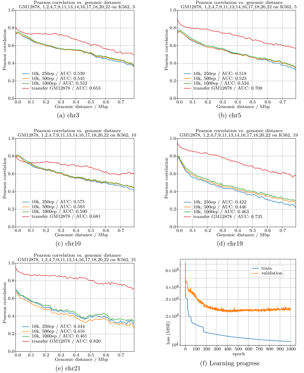
Figure 21: Results / metrics, basic DNN, 10 kbp, test chromosomes
