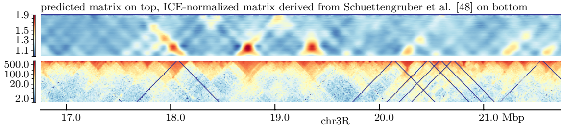
(b) Matrix from DNN, w = 80 , 40 epochs
