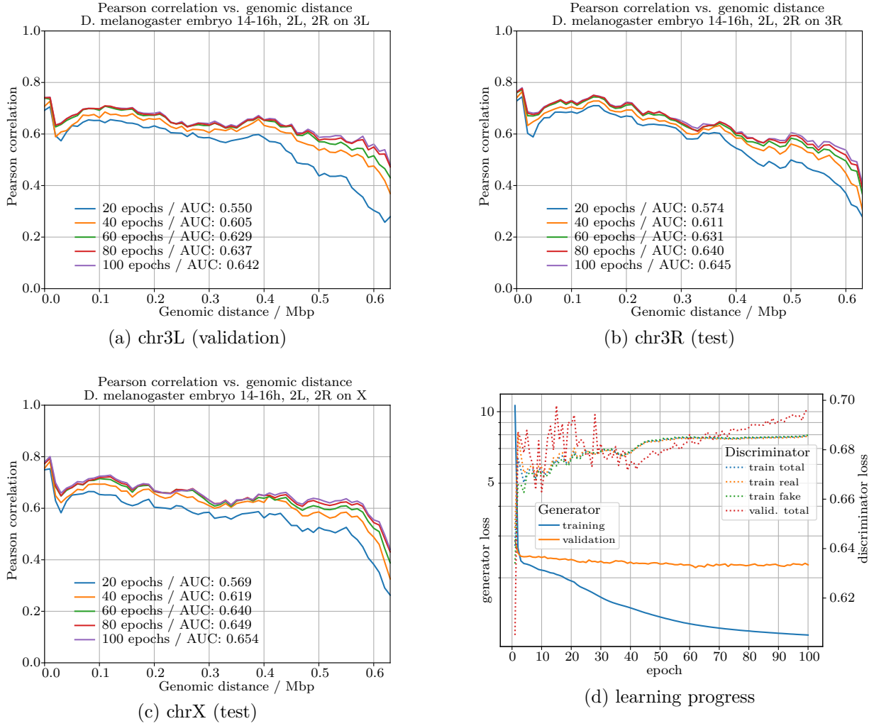
Figure 71: Results / metrics, cGAN, w = 64 , trained on D. Melanogaster chr2L and 2R
