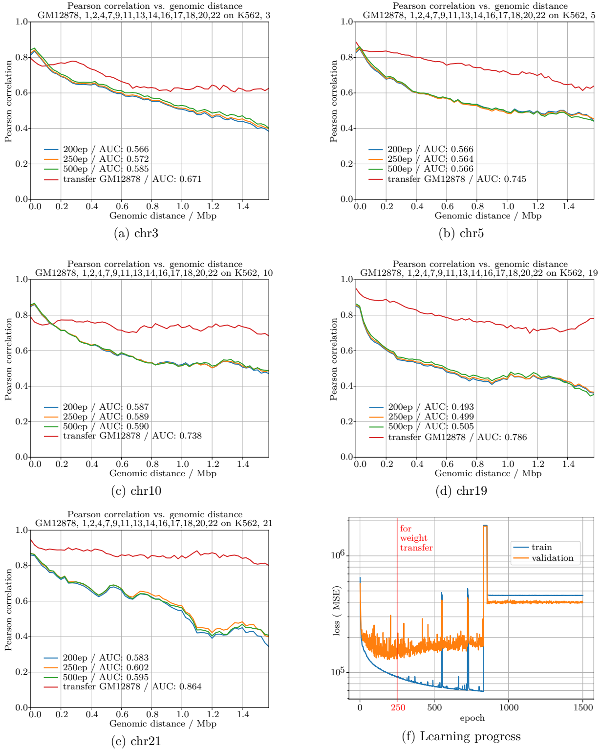
Figure 62: Results / metrics, DNN, w = 64 , test chromosomes
