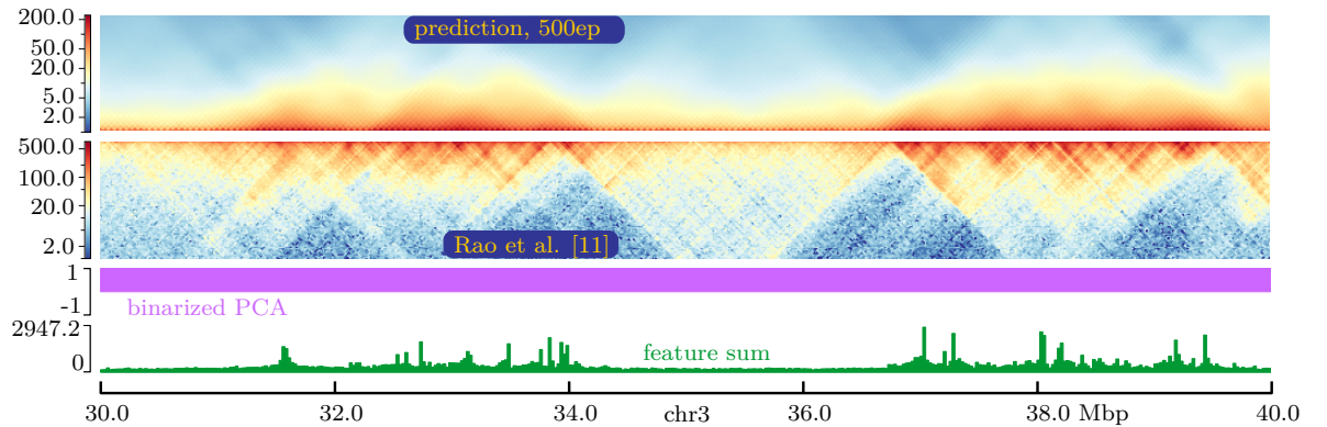
Figure 41: Example predictions GM12878 \rightarrow K562, DNN trained at 25 kbp and 50 kbp simultaneously, 25 kbp, 500 epochs
