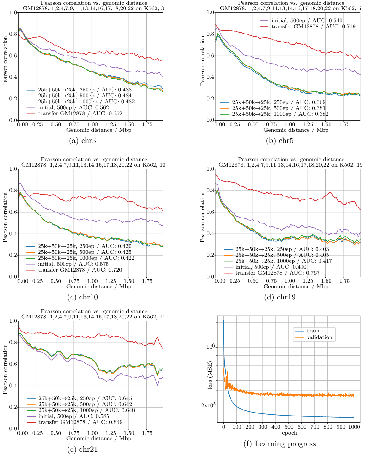
Figure 40: Results / metrics, DNN trained at 25 kbp and 50 kbp simultaneously
