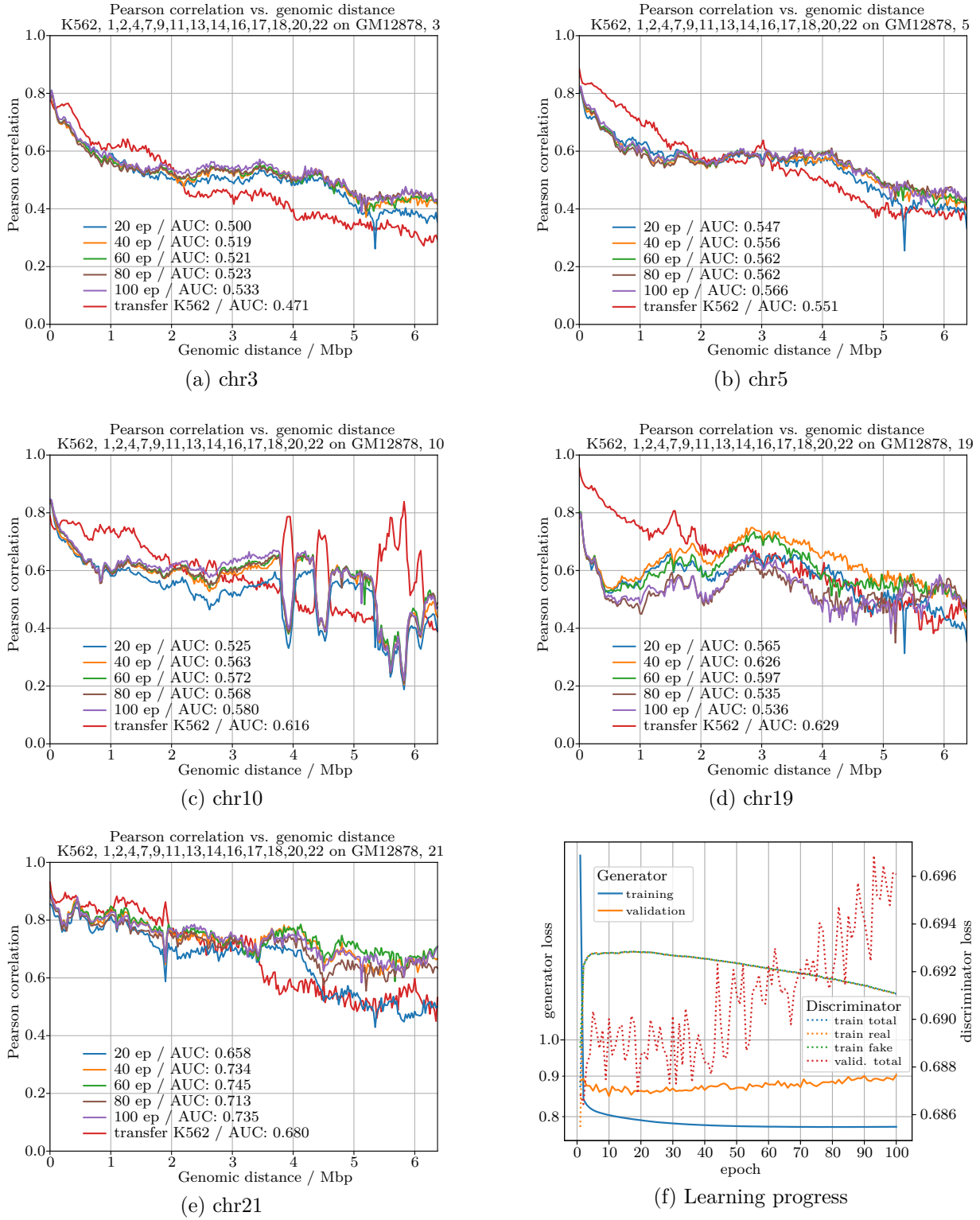
Figure 64: Results / metrics, cGAN, CNN embedding, w = 256 , test chromosomes
