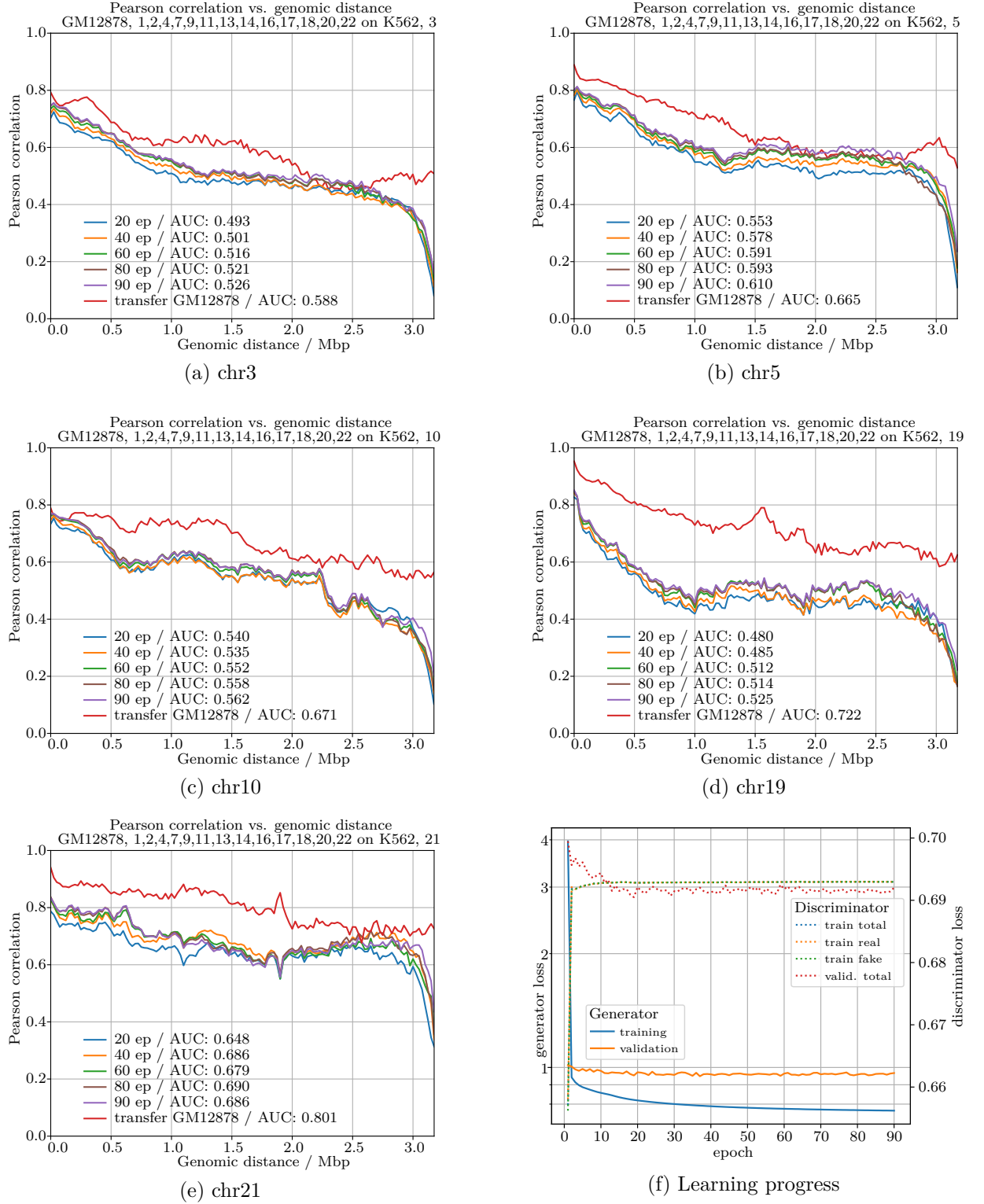
Figure 48: Results / metrics, cGAN, CNN embedding, w = 128 , test chromosomes
