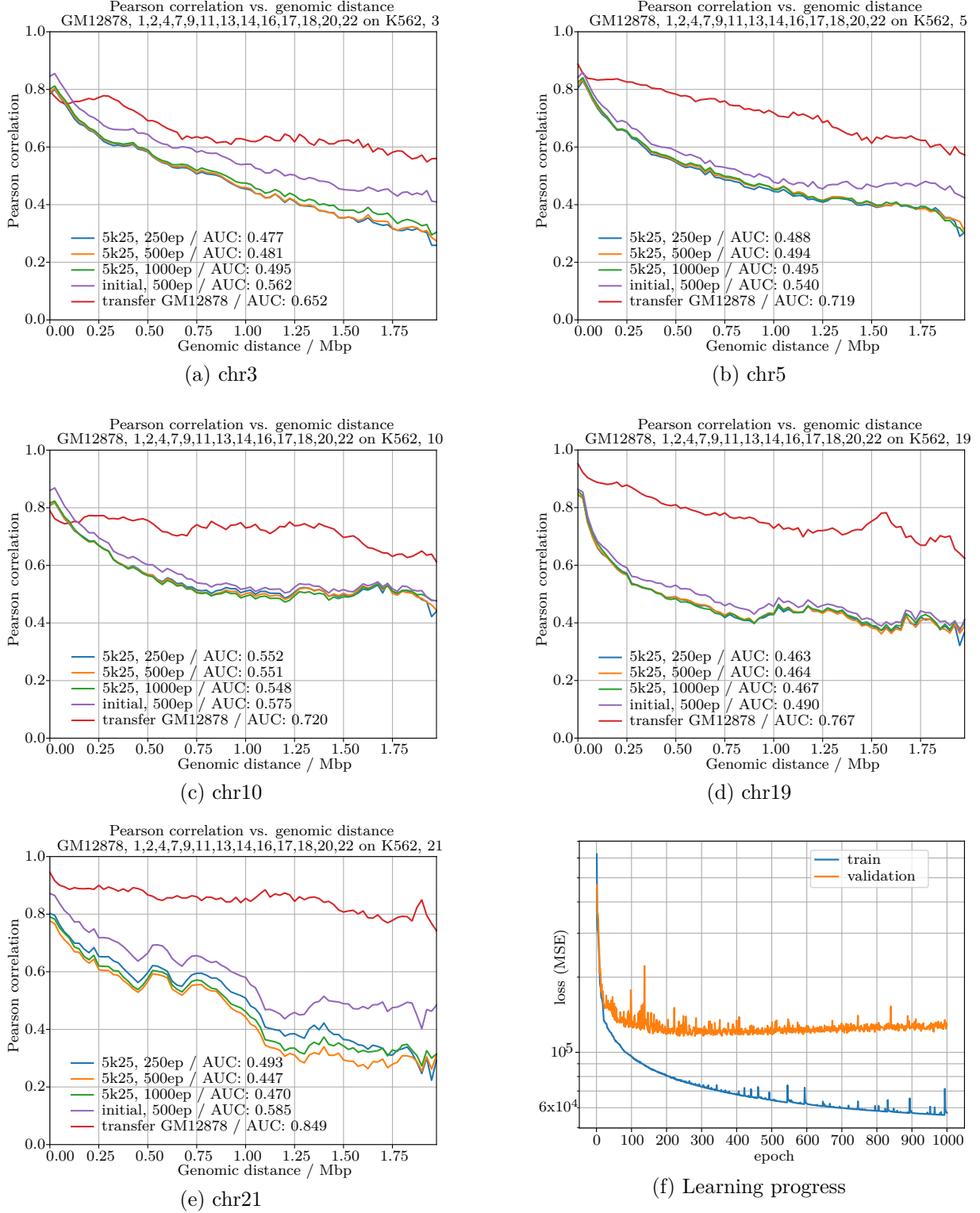
Figure 31: Results / metrics, “5k – 25k” variant of DNN with b_{feat} = 5 kbp and b_{mat} = 25 kbp, test chromosomes
