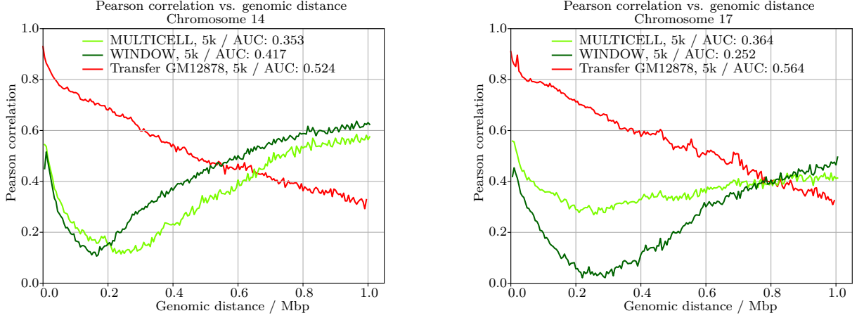
Figure 19: Pearson correlations reconstructed from [28, 82, 83]
