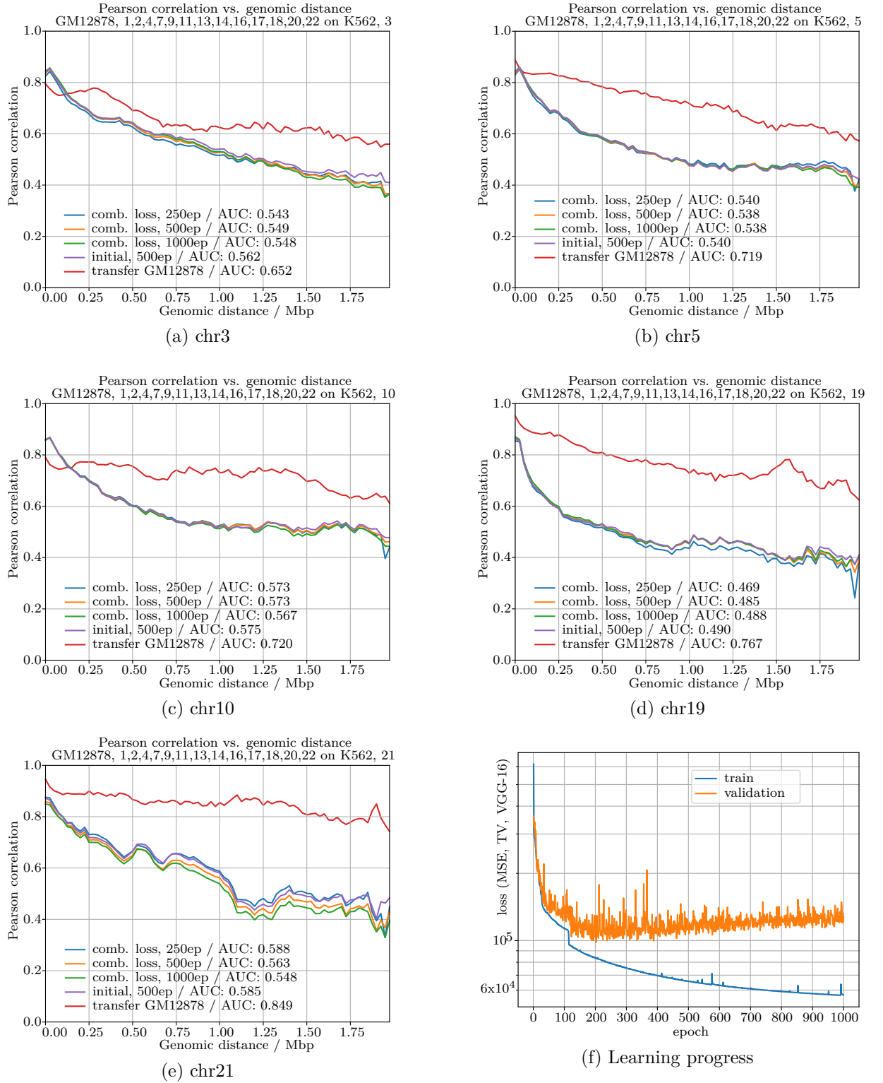
Figure 33: Results / metrics, DNN with combined loss function (MSE, TV, VGG-16), test chromosomes
