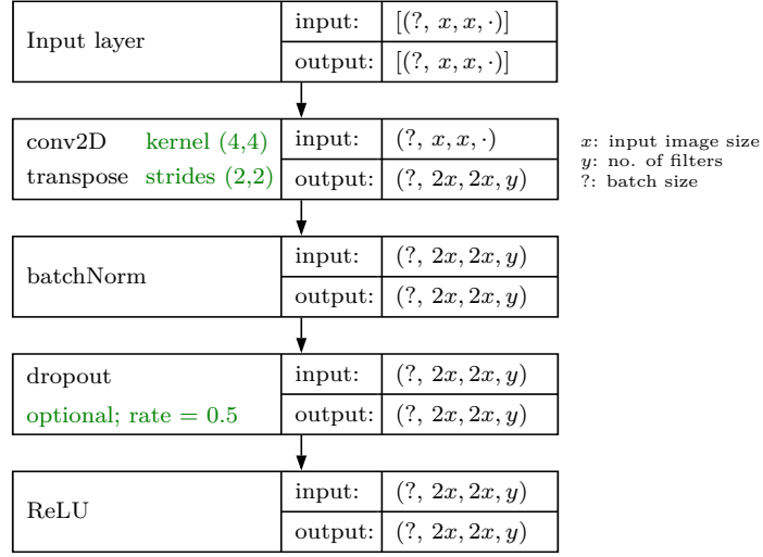
Figure 16: Upsampling block
