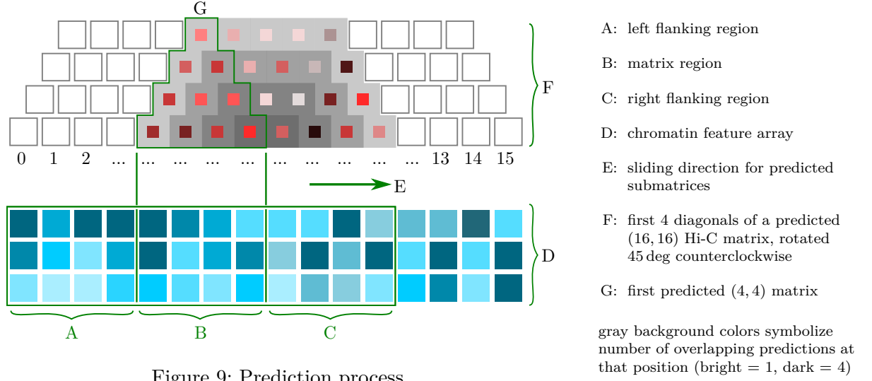
Figure 9: Prediction process
