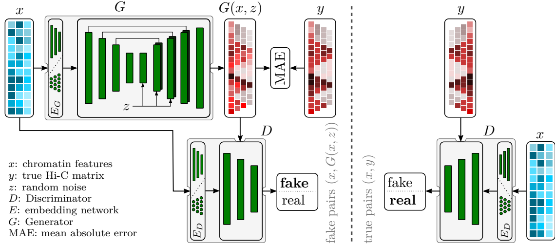
Figure 7: cGAN approach
