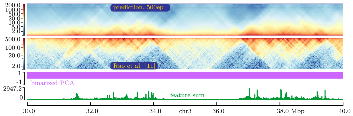
Figure 22: Example predictions GM12878 \rightarrow K562, basic DNN, 25 kbp, 500 epochs
