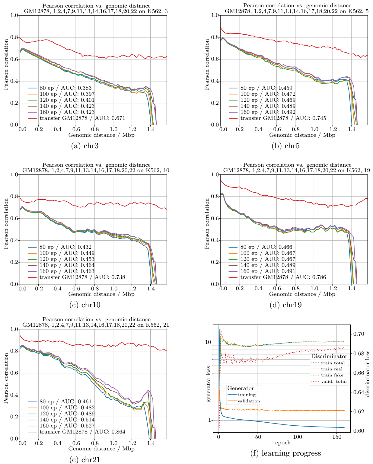
Figure 68: Results / metrics, cGAN, w = 64 , trained on GM12878 chr17 only; prediction on K562, typical test chromosomes
