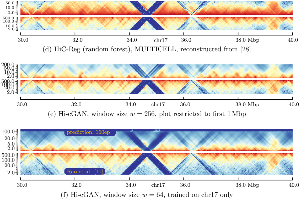
Figure 57: Comparison HiC-Reg [28] and Hi-cGAN (CNN embedding)
