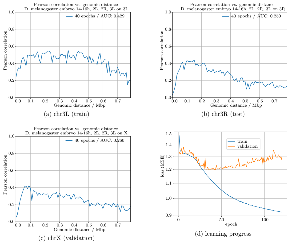
Figure 70: Results / metrics, DNN, w = 80 , trained on D. Melanogaster chr2L, 2R, 3L
