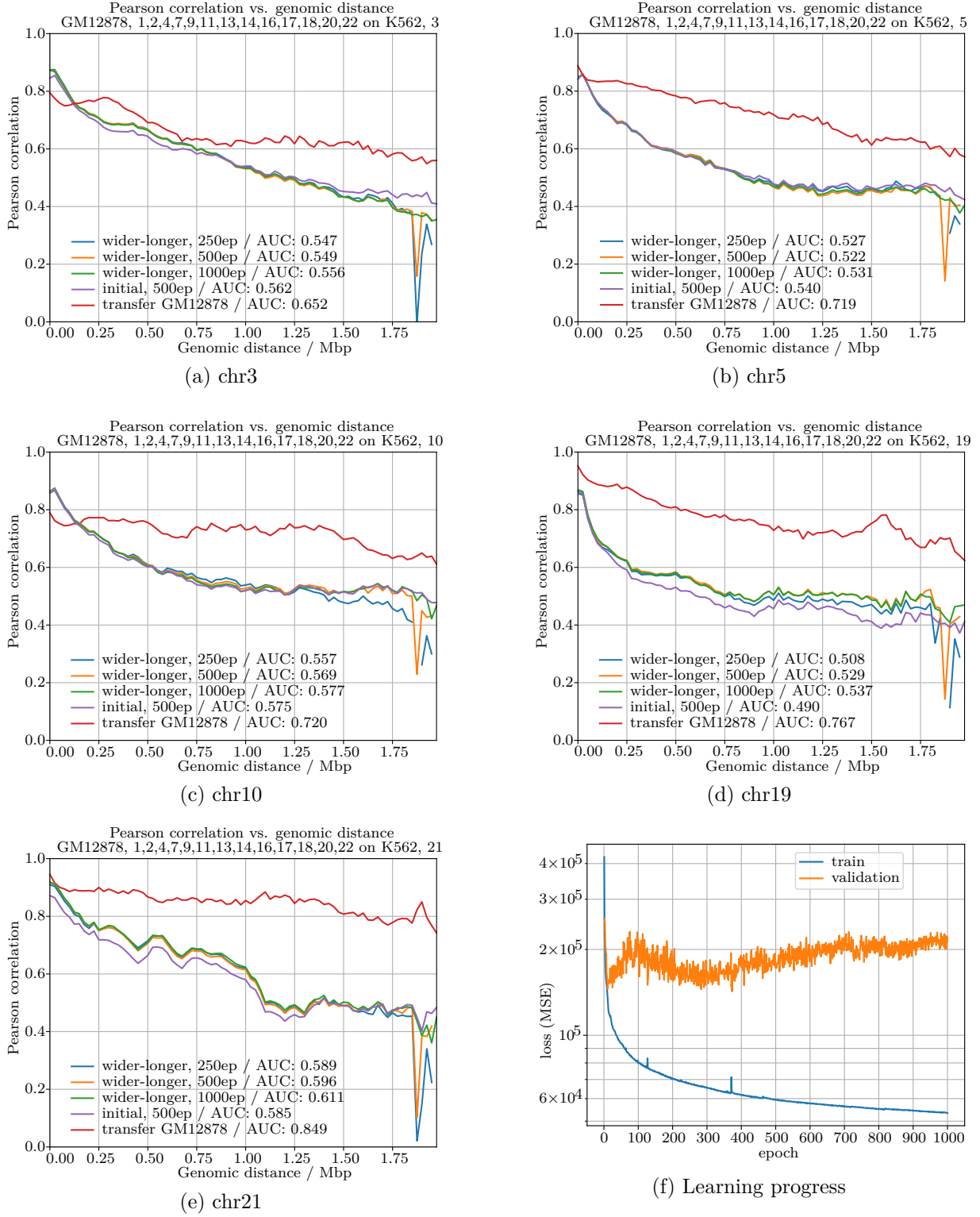
Figure 29: Results / metrics, “wider-longer” variant of DNN, test chromosomes
