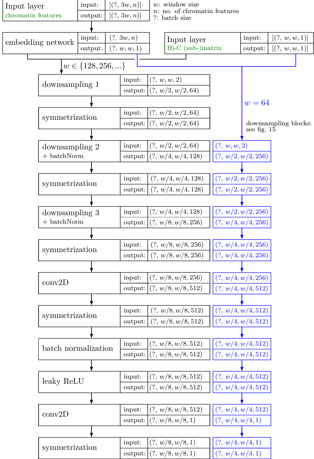
Figure 14: Adapted discriminator model from pix2pix
