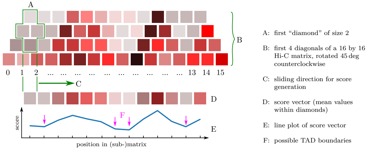
Figure 6: Score vector generation for TAD-based loss
