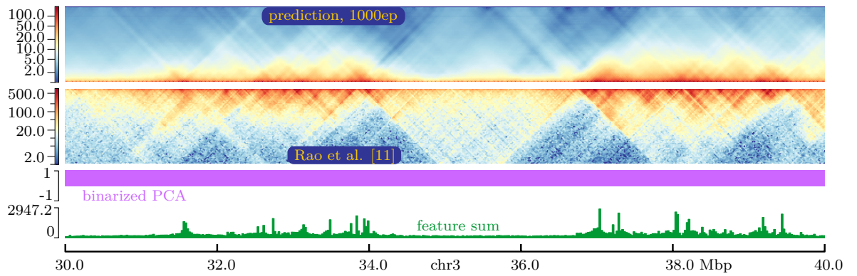
Figure 28: Example predictions GM12878 \rightarrow K562, “wider” variant of DNN, bin size 25 kbp, 1000 epochs
