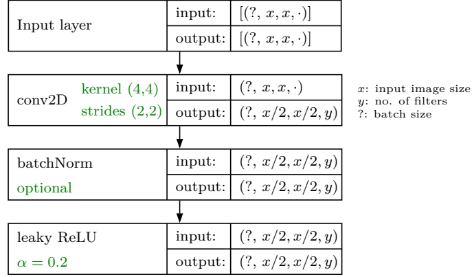
Figure 15: Downsampling block
