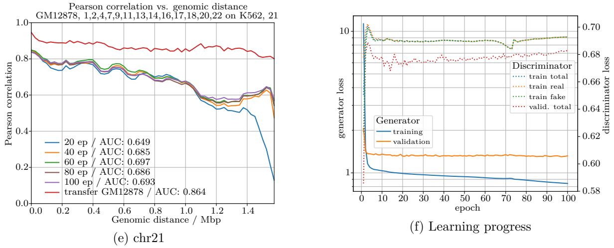
Figure 66: Results / metrics, cGAN, w = 64 , trained on GM12878 chr14 only; prediction on K562, typical test chromosomes
