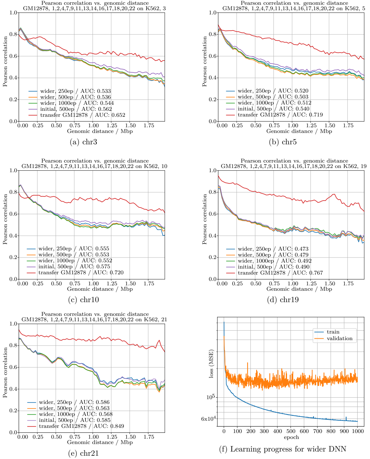
Figure 27: Pearson correlations, “wider” variant of DNN, test chromosomes
