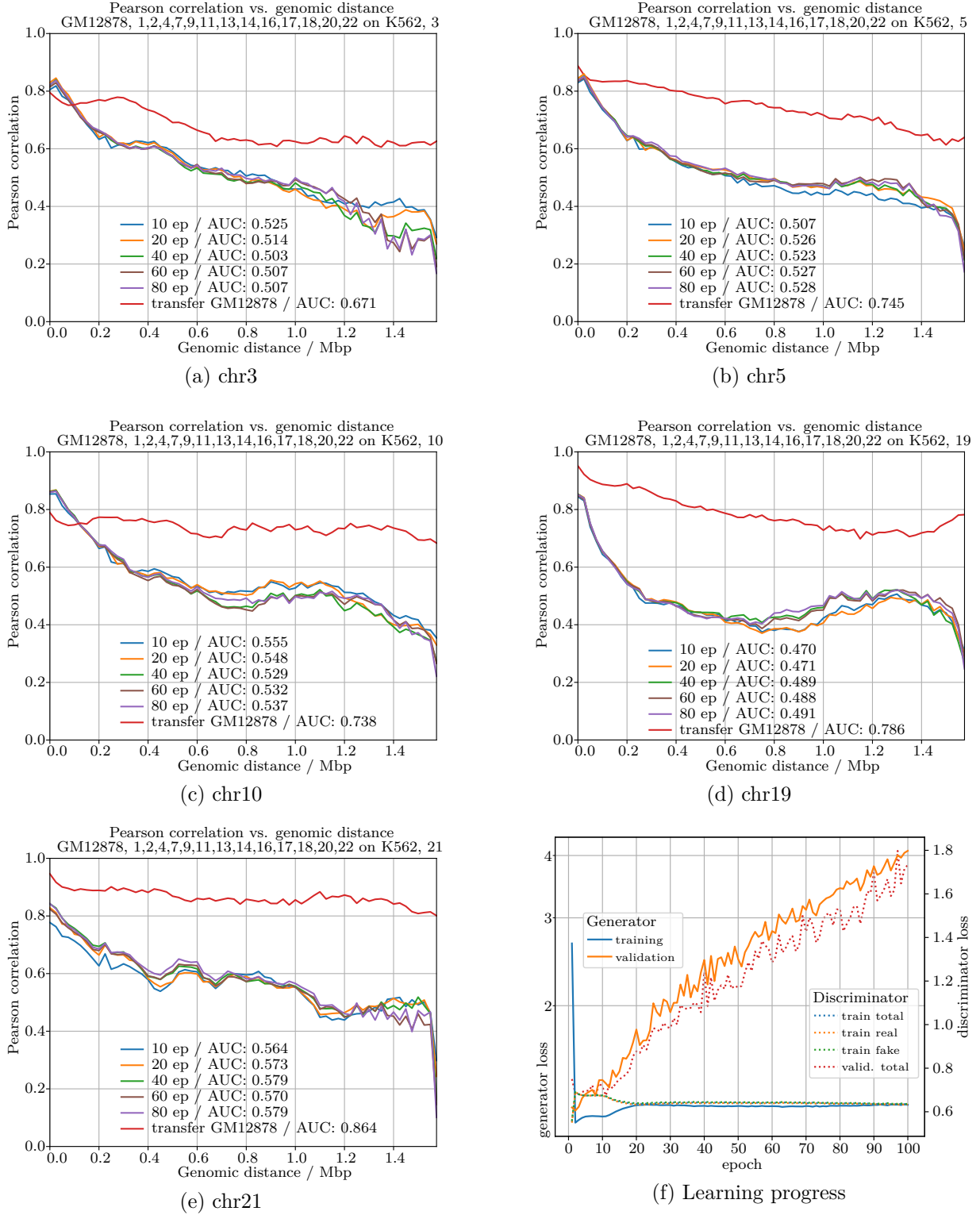
Figure 54: Results / metrics, cGAN, mixed embedding, DNN pre-trained, w = 64 , test chromosomes
