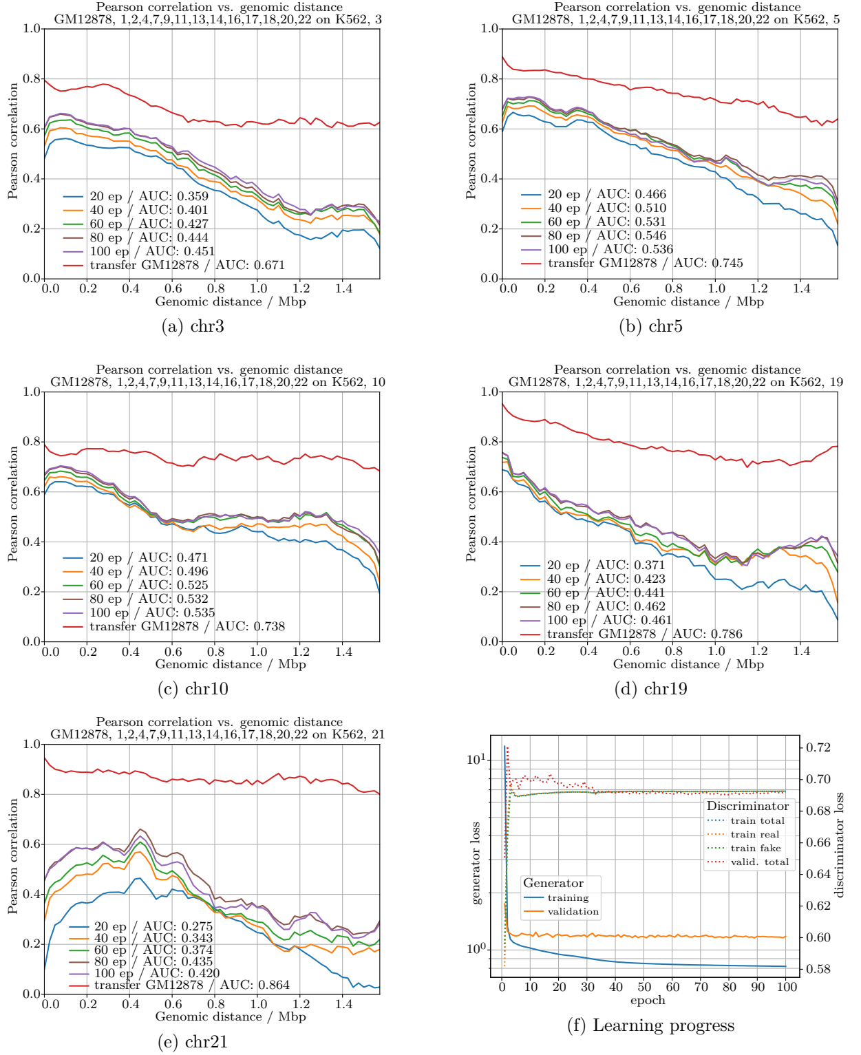
Figure 46: Results / metrics, cGAN, CNN embedding, w = 64 , test chromosomes
