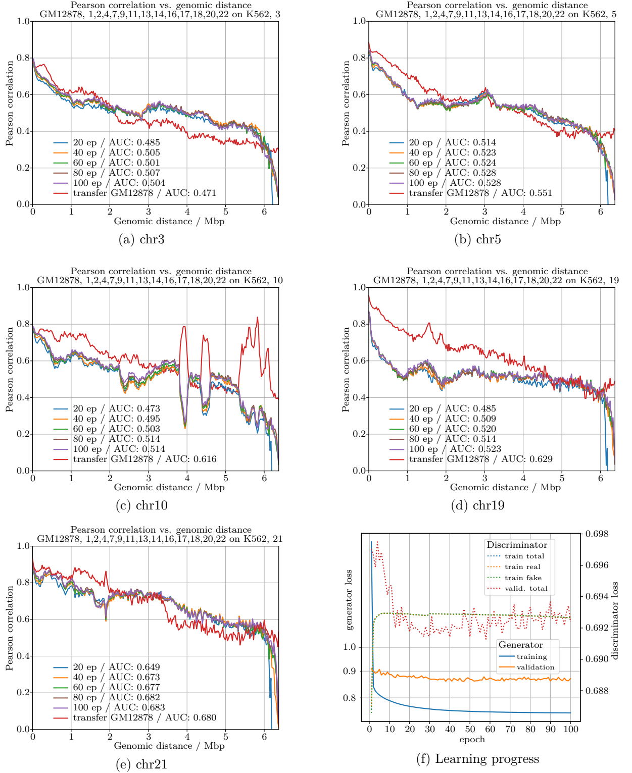
Figure 50: Results / metrics, cGAN, CNN embedding, w = 256 , test chromosomes
