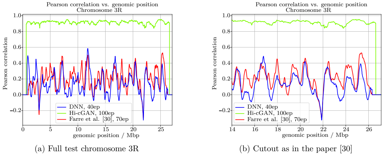
Figure 58: Comparison Pearson correlations per position DNN / Hi-cGAN / Farré et al. [30]
